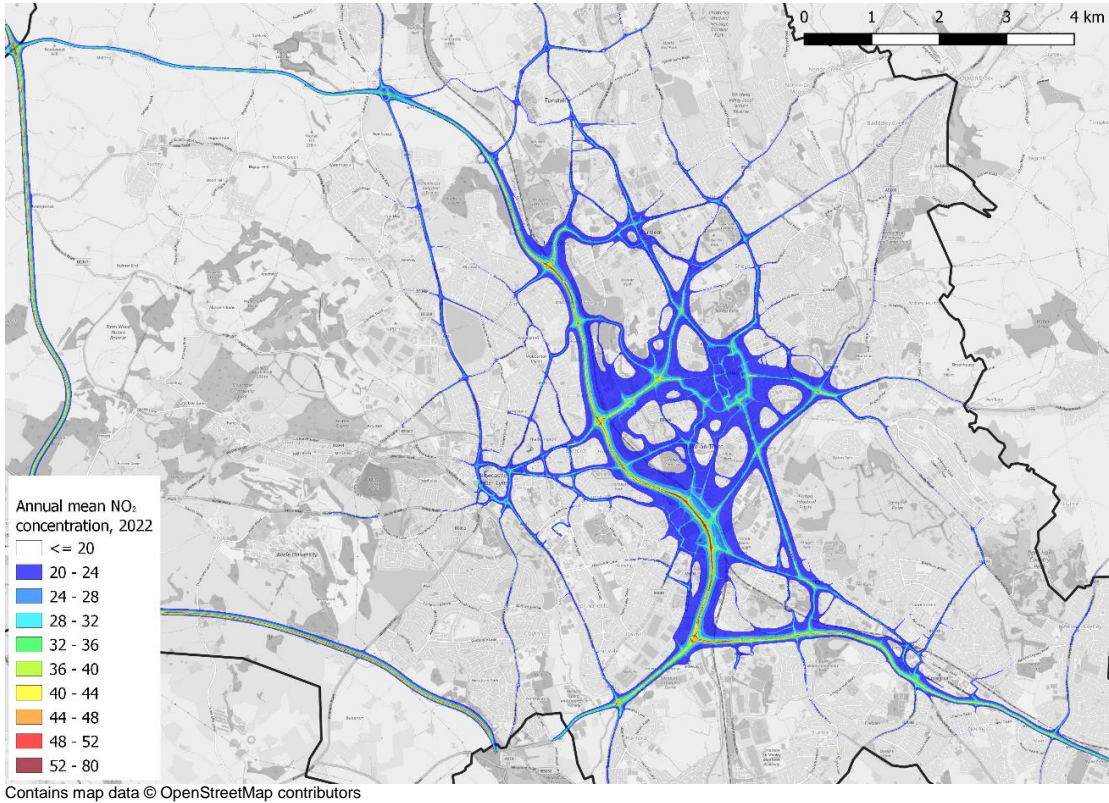
Figure 3-4: Annual mean NO 2 concentrations, 2022, \mu\text{g}\cdot\text{m}^{-3} , study domain
