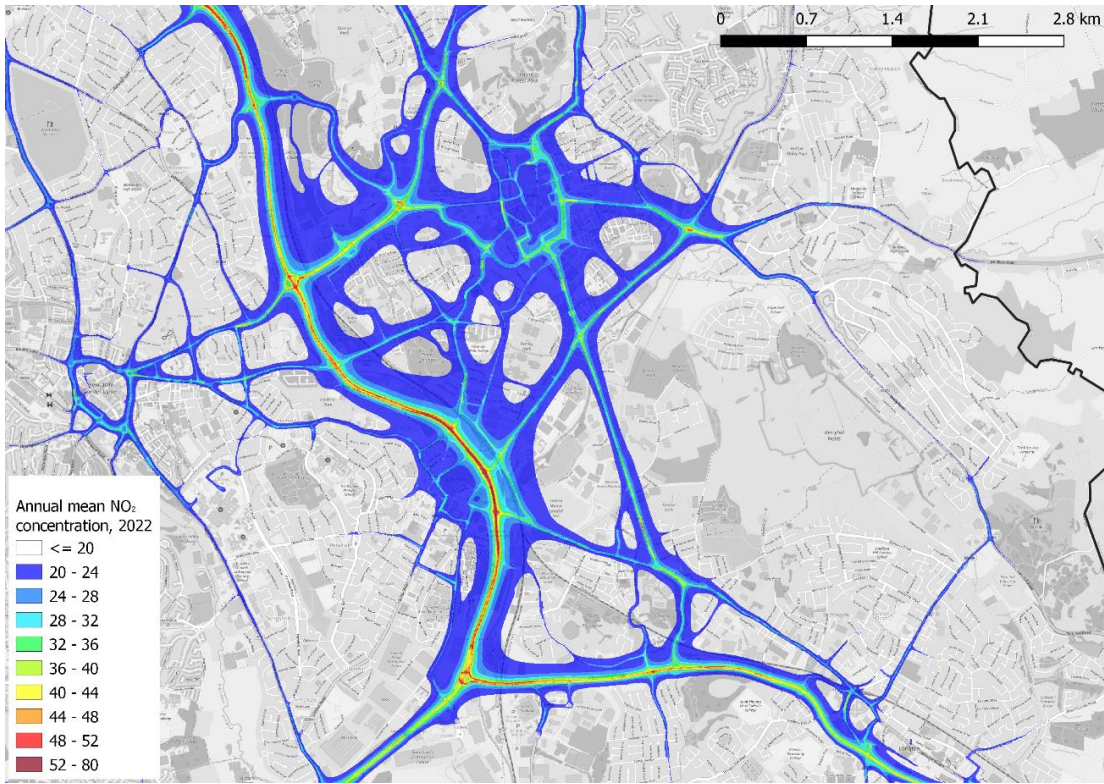
Figure 3-6 Annual mean NO 2 concentrations, 2022, µg.m -3 , Hanley
