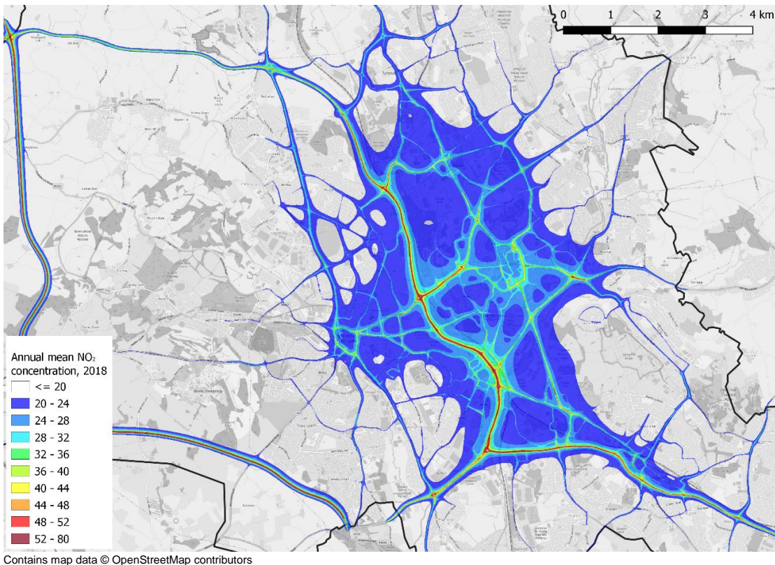
Figure 3-2: Annual mean NO 2 concentrations, 2018, µg.m -3 , model domain
