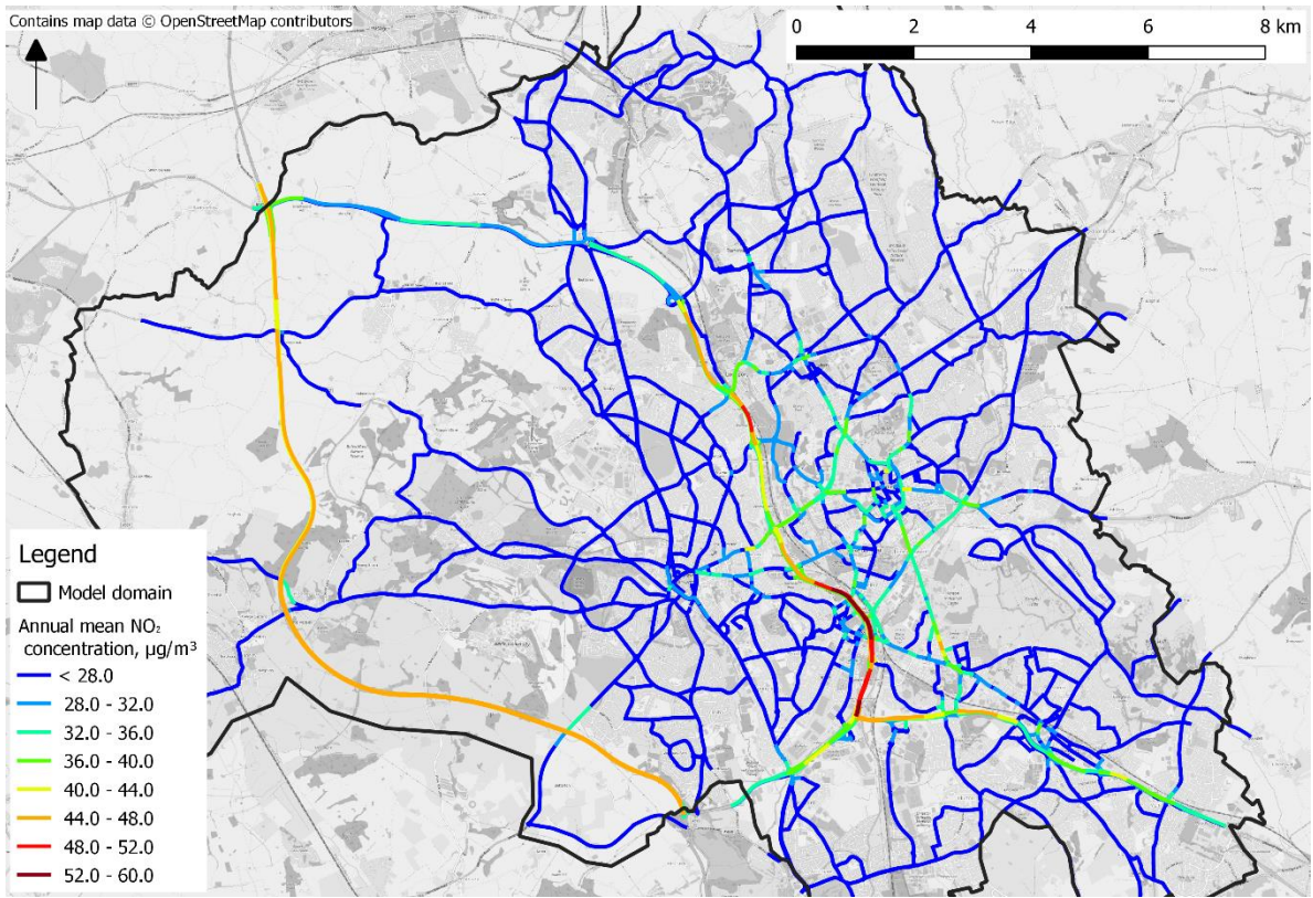
Figure 3-4: Annual mean NO 2 concentrations, 2022, \mu\text{g}\cdot\text{m}^{-3} , study domain
