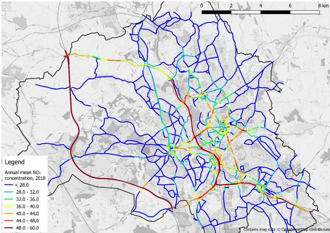
Figure 3-2: Annual mean NO 2 concentrations, 2018, µg.m -3 , model domain
